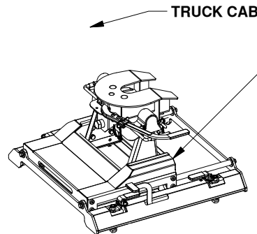
Figure H3: View of Slider Base with the Carriage in a forward position. TOWING POSITION
