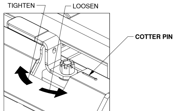
FIGURE B4: View of base leg.
