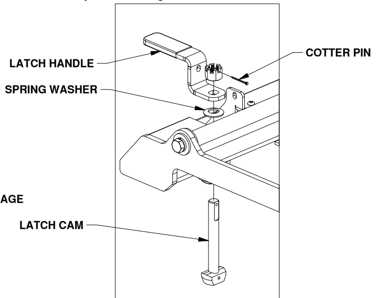
FIGURE B3: List of latch parts.
