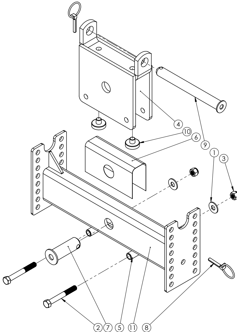
6331 Parts List
