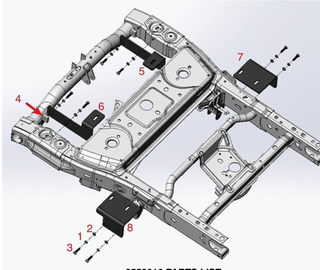
8553016 PARTS LIST
