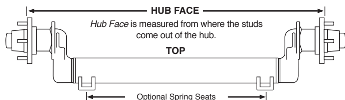
4" Drop Axle
