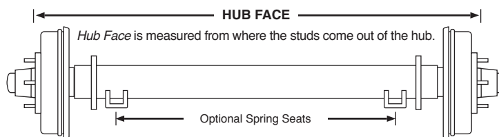
Straight Axle
