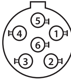
603P (6-Pole)
